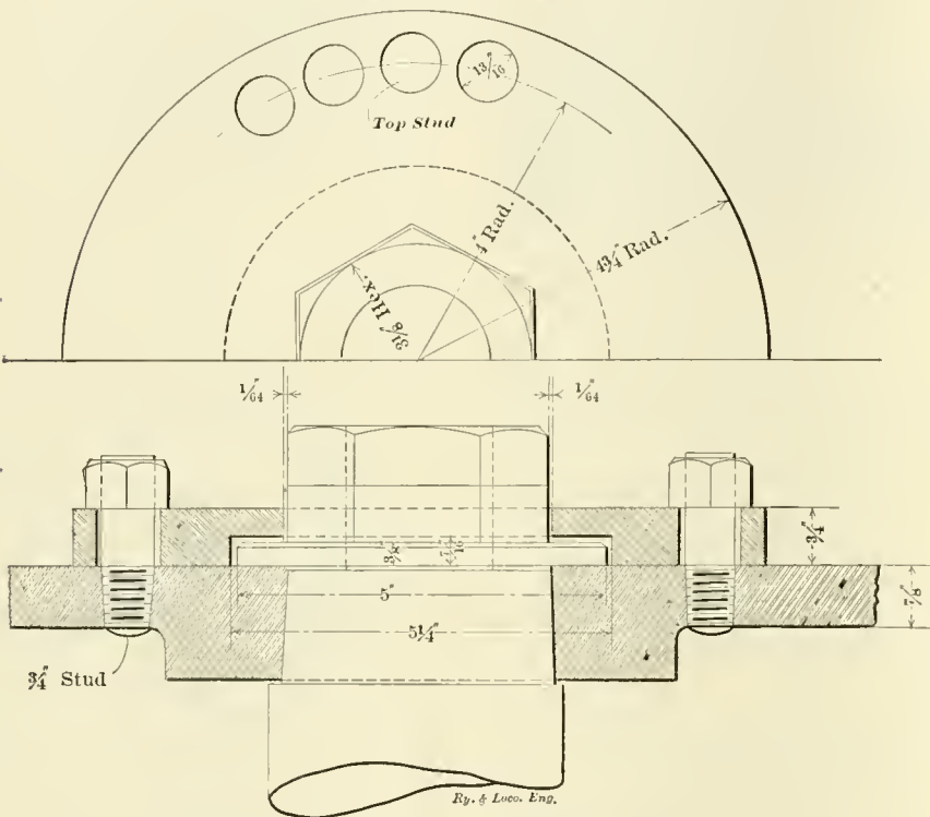
WRIST PIN NUT LOCK.
